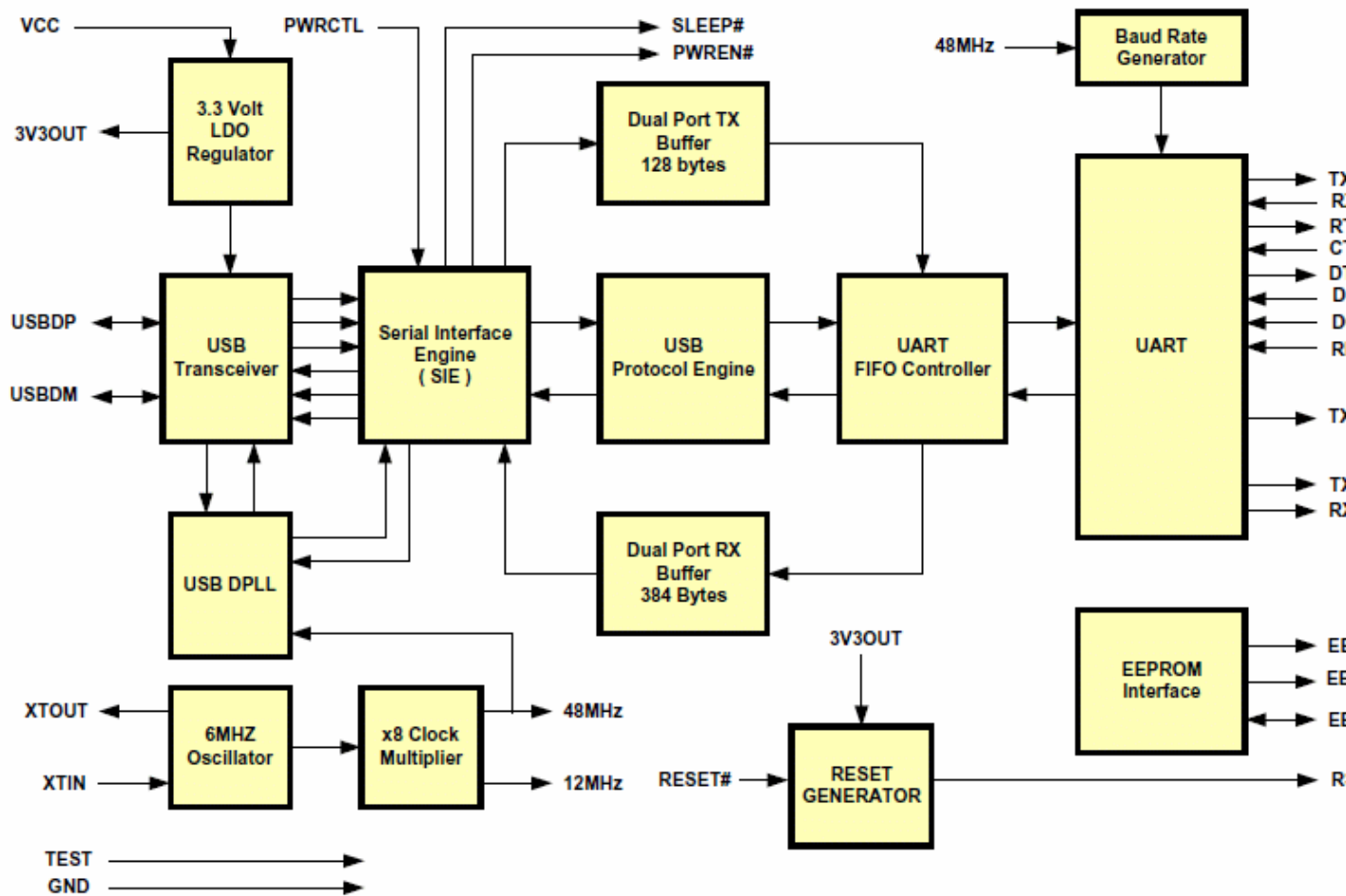
Figure 2.1 FT232BM Block Diagram
