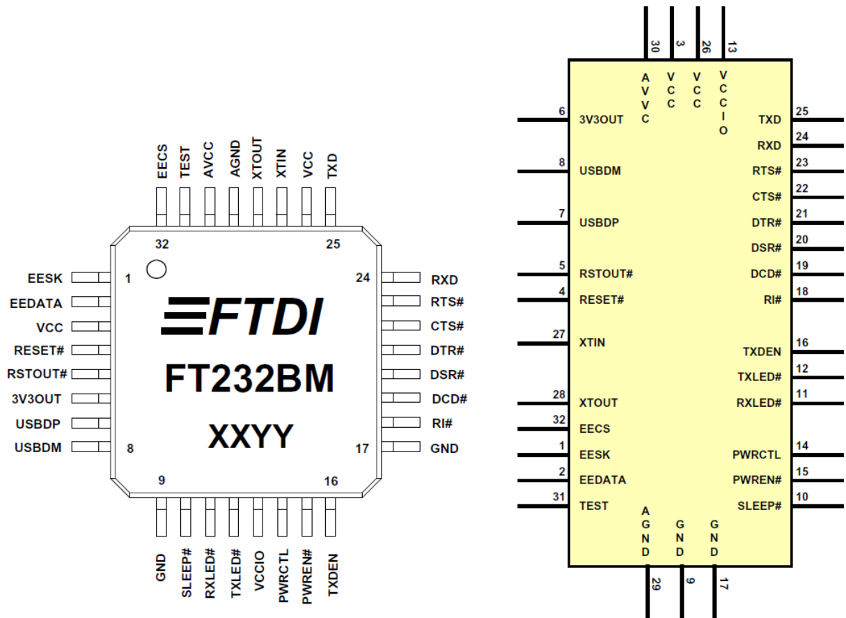
Figure 3.1 LQFP Package Pin Out and Schematic Symbol
