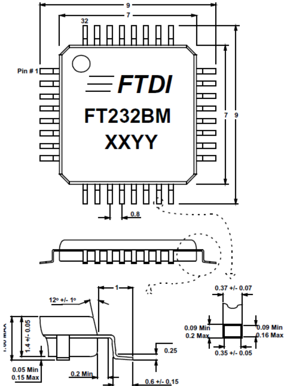
Figure 11.1 32 LQFP Package Dimensions
