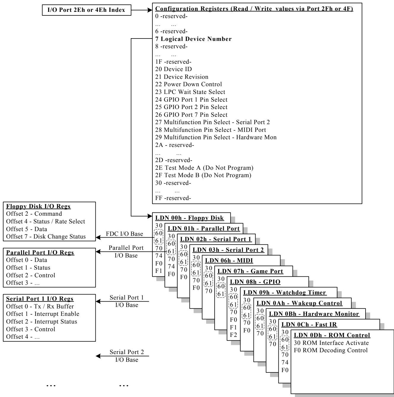
Figure 3. Register Map
