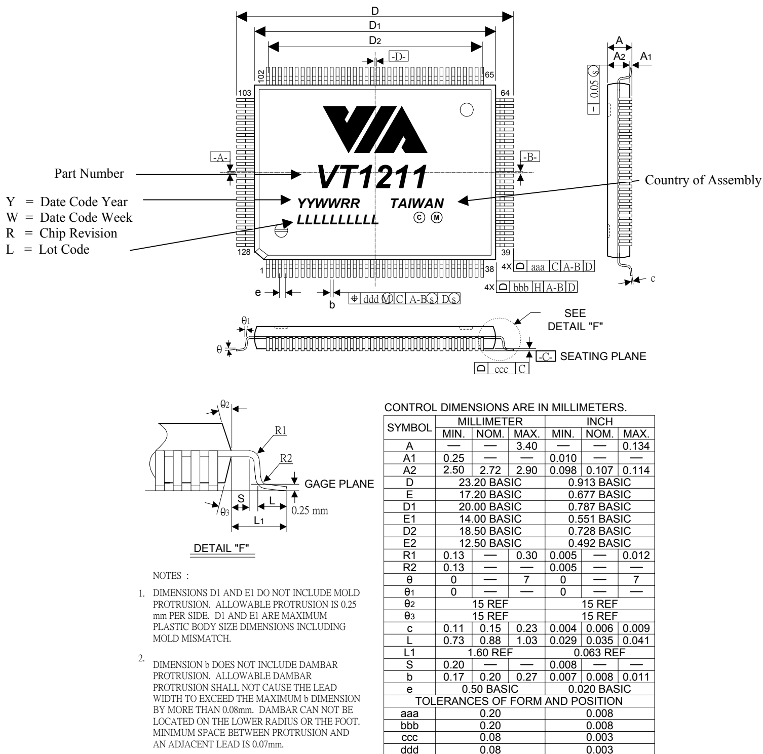
Figure 6. 128-Pin PQFP – Plastic Quad Flat Pack
