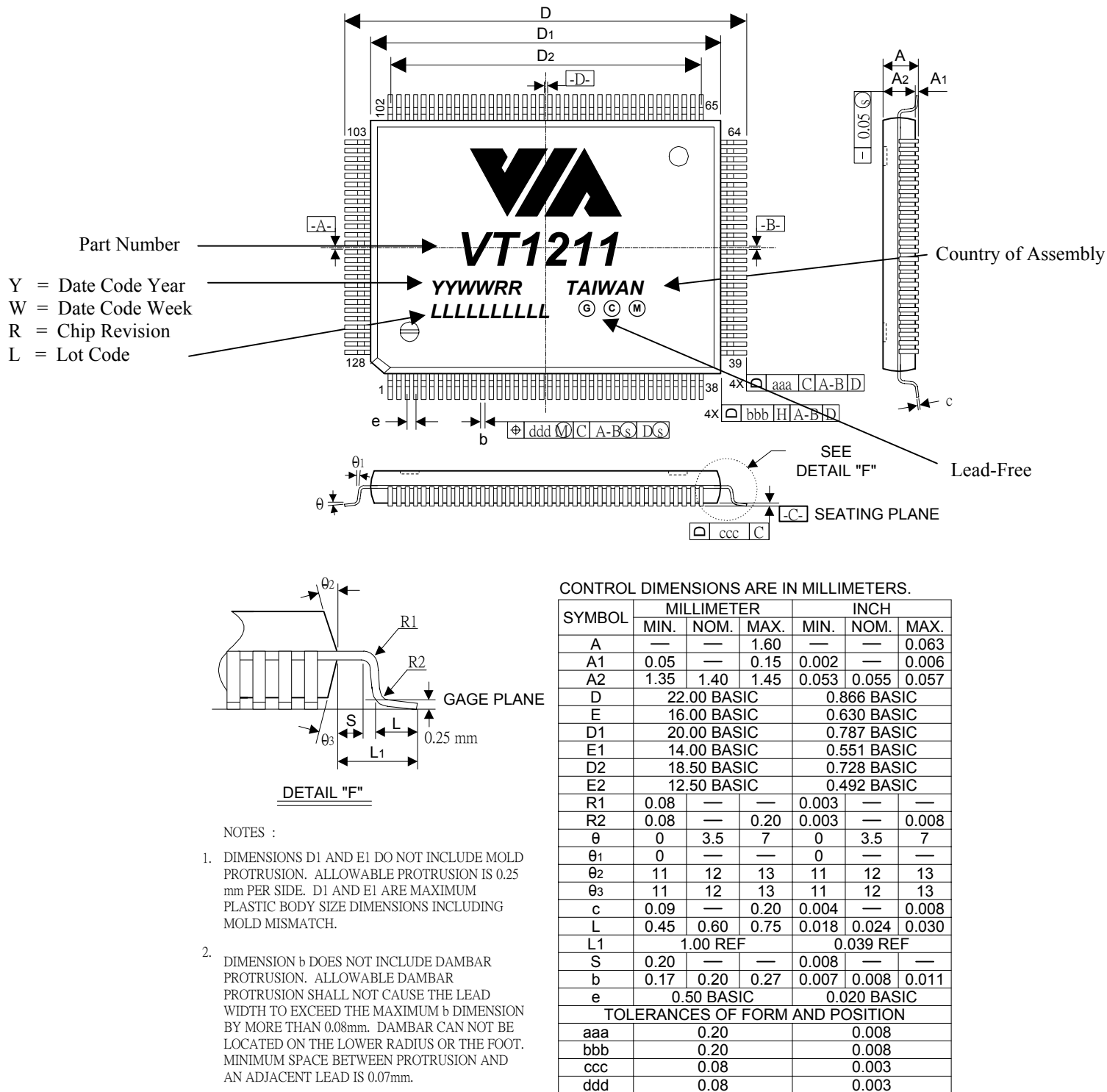
Figure 5. 128-Pin LQFP – Lead-Free Low-Profile Quad Flat Pack
