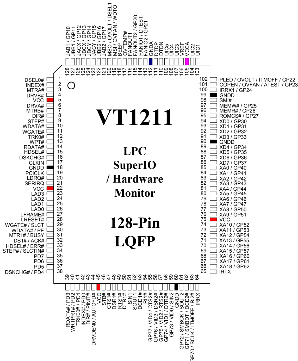
Figure 1. VT1211 Pin Diagram (Top View)
