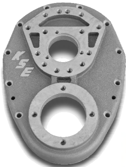
KSD1002 Front Cover, Aluminum Standard Cam Position
