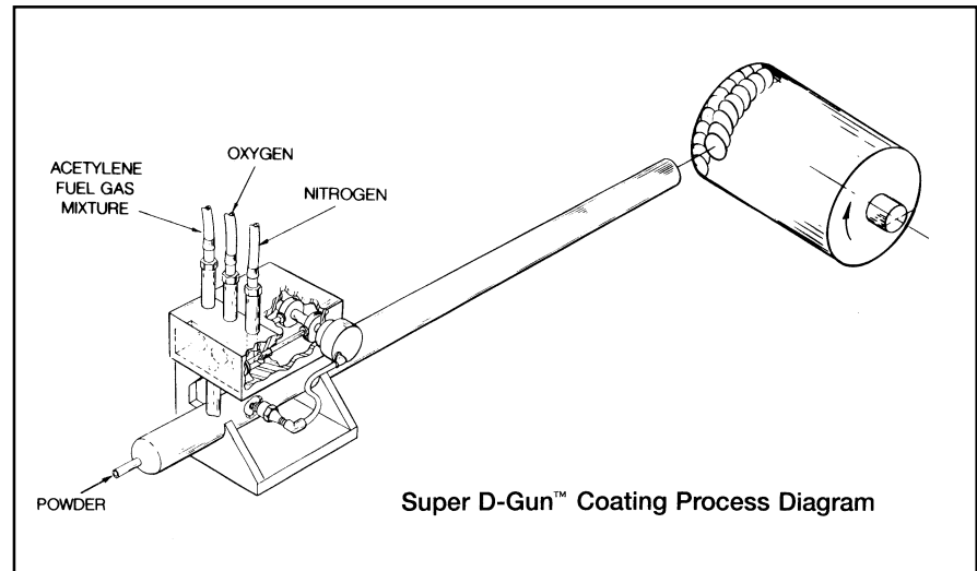
Schematic of the Super D-Gun™ Process
