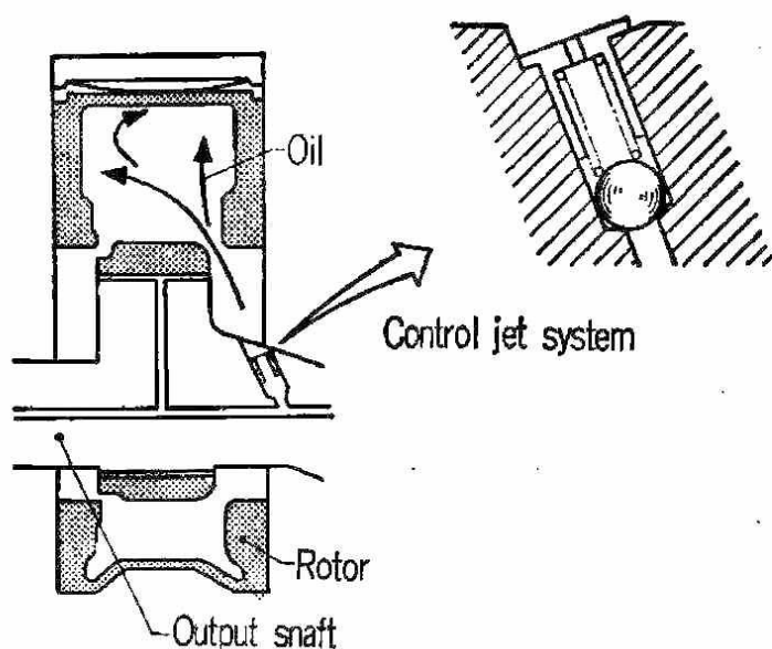
Control of lubricating oil injection
