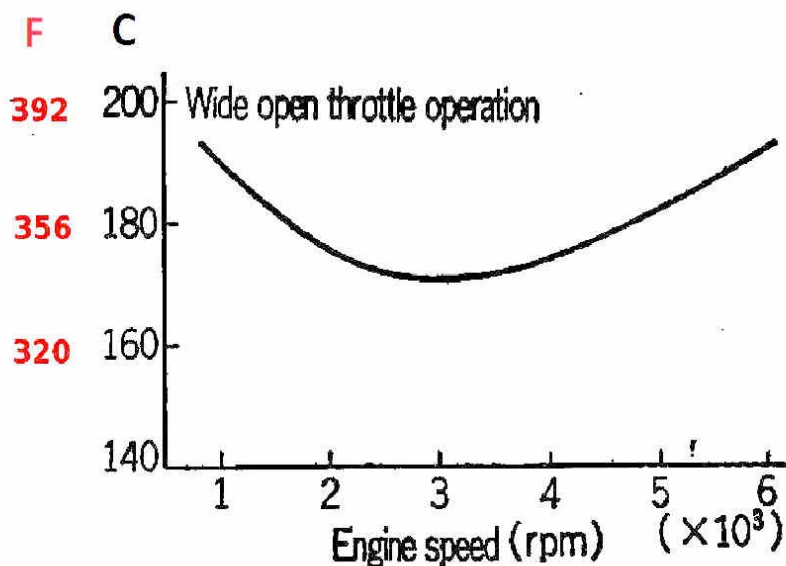
Change in rotor surface temperature
