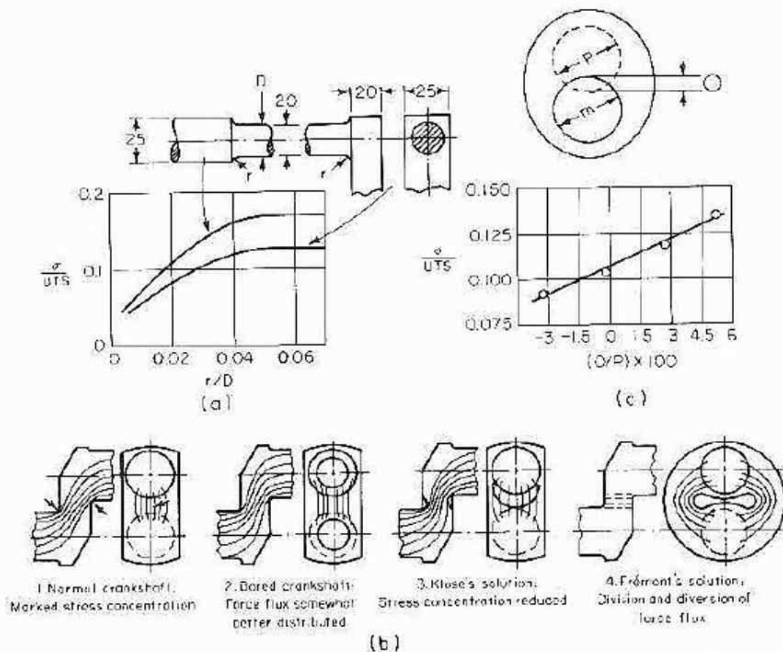
Fig. 11-35. Crank stress patterns (Matinaglia, 11.700). (a) Endurance-limit nominal stress in torsion ( \sigma ) versus fillet radius. Numbers are dimensions of test pieces in cm; (b) "flux" of force from pin to journal. Stress is smaller as flux lines are farther apart. (c) Effect of overlap on crank endurance strength in bending. The dimensions held constant, in millimeters are as follows: Crank throw 73; pin length 52; pin bore 40; journal length 37; journal bore 50; cheek thickness 22; cheek width 126. The dimensions varied, in millimeters, were as follows:
